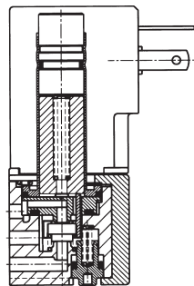
3/2 - NC
